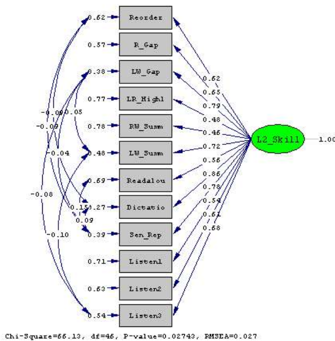
Figure 1. A one-factor model
